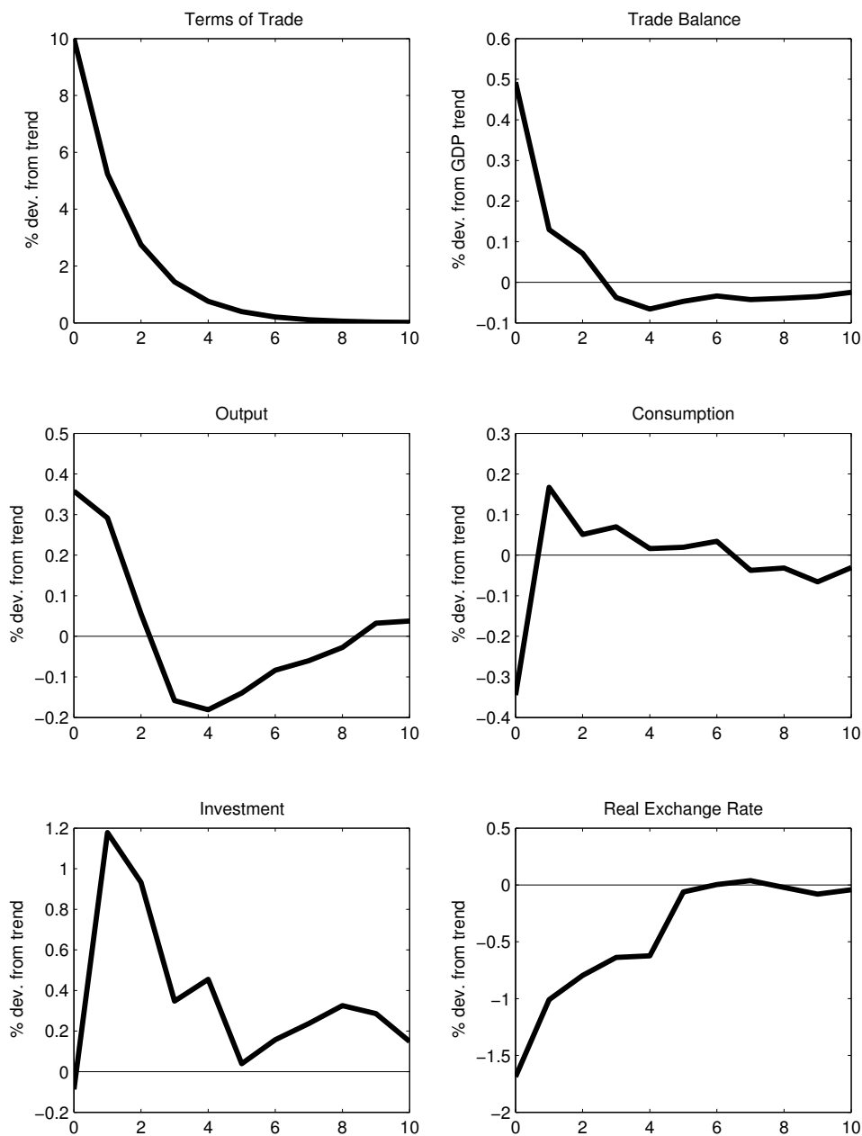
Figure 1: Impulse Response to An Innovation in the Terms of Trade: SVAR Evidence
