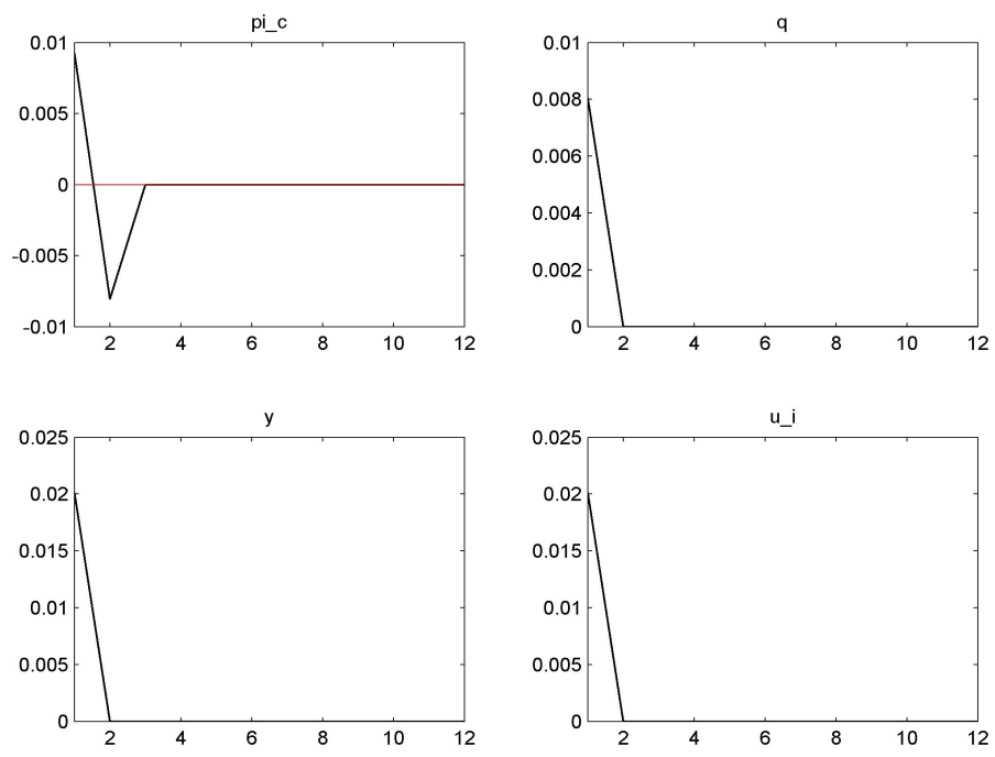
Figure 5: The impulse response function of e_{it} on macroeconomic variables
