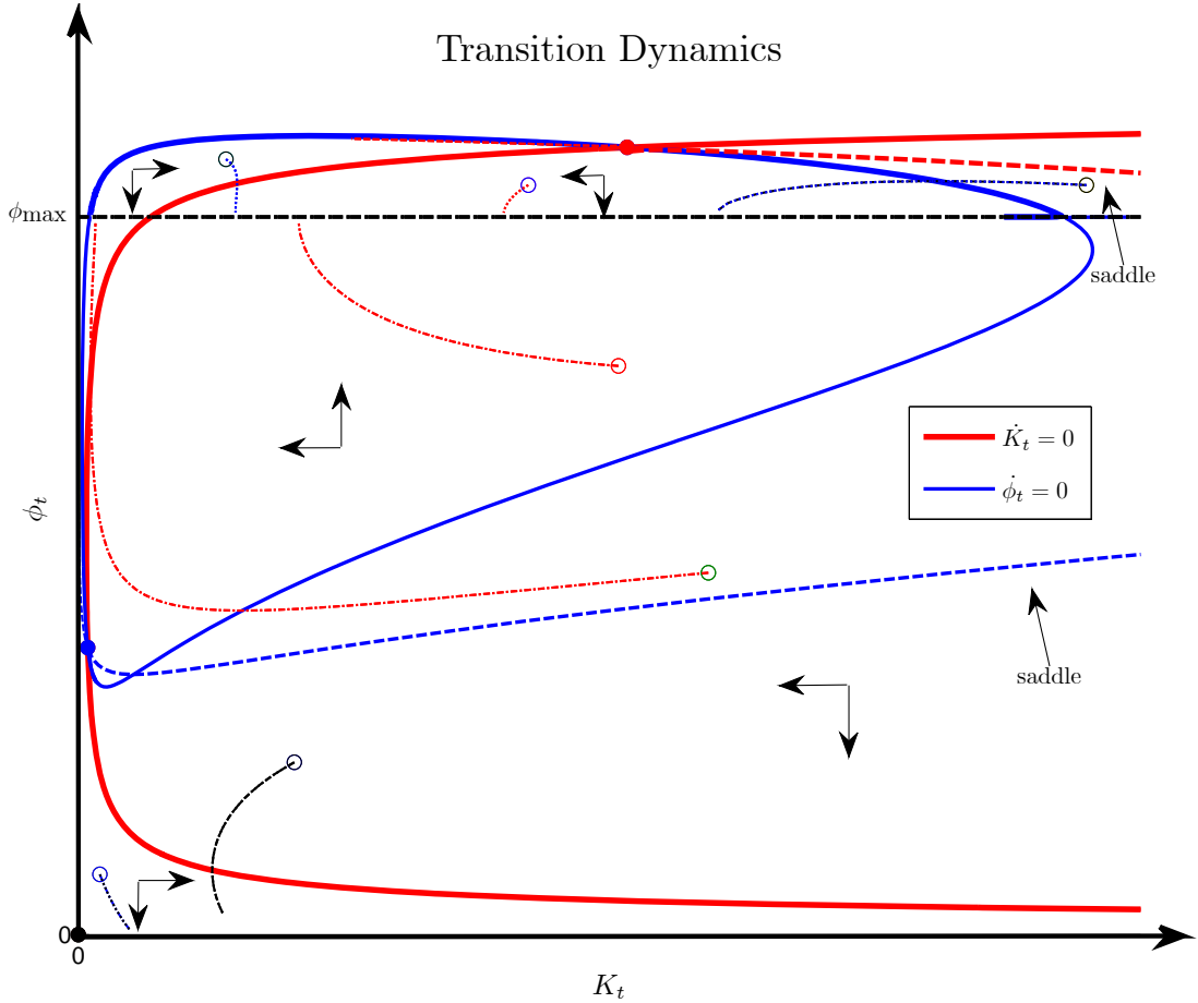
Figure 4: Global Dynamics with One Saddle: Relatively High \pi (we set \alpha = 0.62 and \Phi = 22 , while all other parameter values are from Table 1.)
