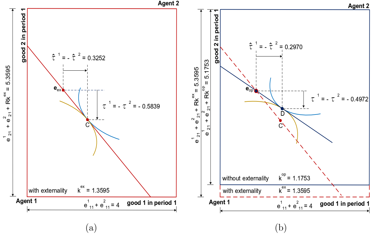
Figure 2: (a) Point C is the competitive collateral equilibrium allocation (with externality) in period t = 1 with \mathbf{c}_1^1 = (1.3252, 1.7756) and \mathbf{c}_1^2 = (2.6748, 3.5839) . An agent type 1 buys 0.3252 units of good 1, sells 0.5839 units of good 2 at price p(z^{\text{ex}}) = 0.5570 in spot markets, and vice versa. Note that \mathbf{e}_{\text{ex}} is the pre-trade allocation (with externality) in period t = 1 . (b) Point D is the competitive equilibrium with segregated security exchanges allocation (without externality) in period t = 1 with \mathbf{c}_1^1 = (1.2970, 1.6781) and \mathbf{c}_1^2 = (2.7030, 3.4972) . An agent type 1 buys 0.2970 units of good 1, sells 0.4972 units of good 2 at price p(z^{\text{op}}) = 0.5974 in spot markets, and vice versa. Note that \mathbf{e}_{\text{op}} is the pre-trade allocation (without externality) in period t = 1 .
