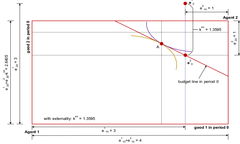
Figure 1: Point A is the competitive collateral equilibrium allocation (with externality) in period t = 0 with \mathbf{c}_0^1 = (2.6899, 1.7756) and \mathbf{c}_0^2 = (1.3101, 0.8649) . An agent type 1 sells 0.3101 units of good 1, buys 0.1128 units of good 2, and k^{ex} = 1.3595 saves units of good 2, and vice versa.
