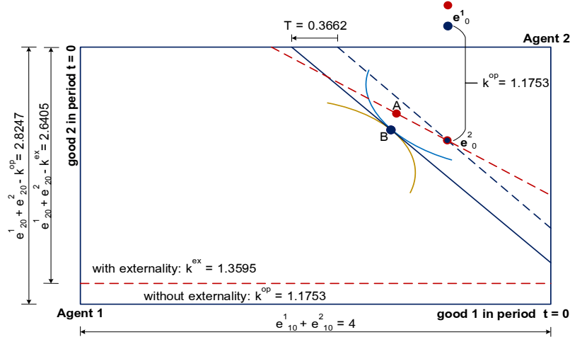
Figure 3: Point B is the competitive collateral equilibrium allocation (without externality) in period t = 0 with \mathbf{c}_0^1 = (2.6073, 1.8410) and \mathbf{c}_0^2 = (1.3927, 0.9837) . where an agent type 1 sells 0.3927 units of good 1, buys 0.0163 units of good 2, and k^{op} = 1.1753 saves units of good 2, and vice versa.
