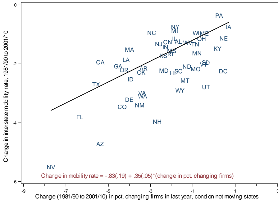
Job Changes Conditional on Not Changing States and Changes in In-Migration
