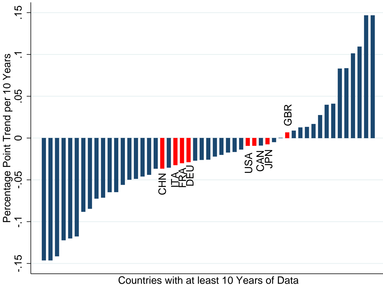
Figure 4: Estimated Trends in Corporate Labor Shares
