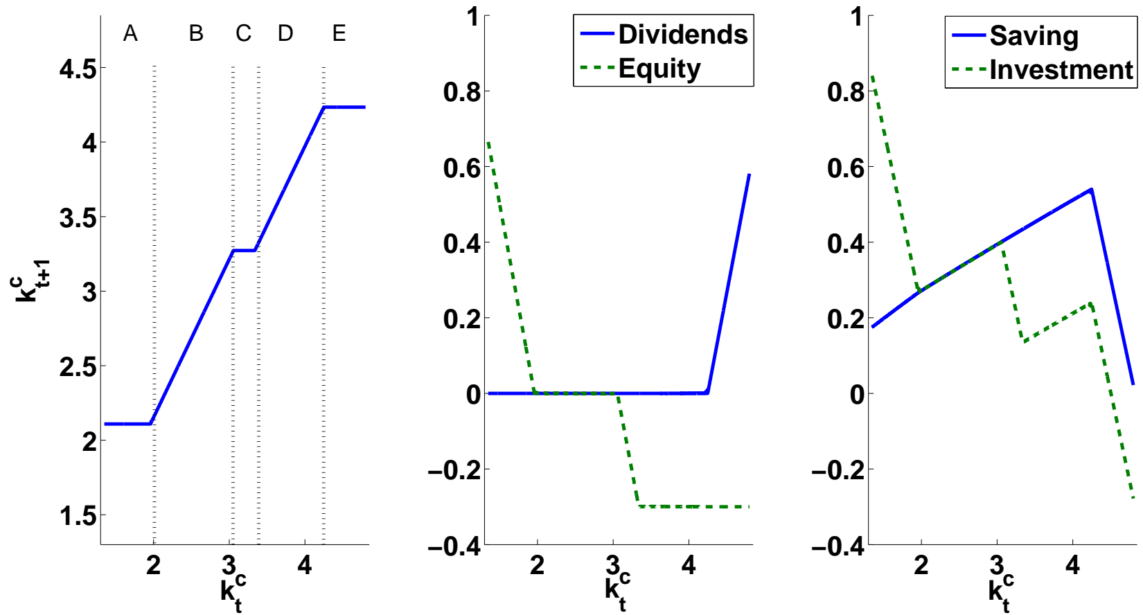
Figure 10: Policy Functions
