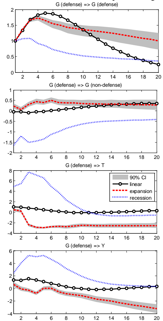
confidence bands for the expansion regime
