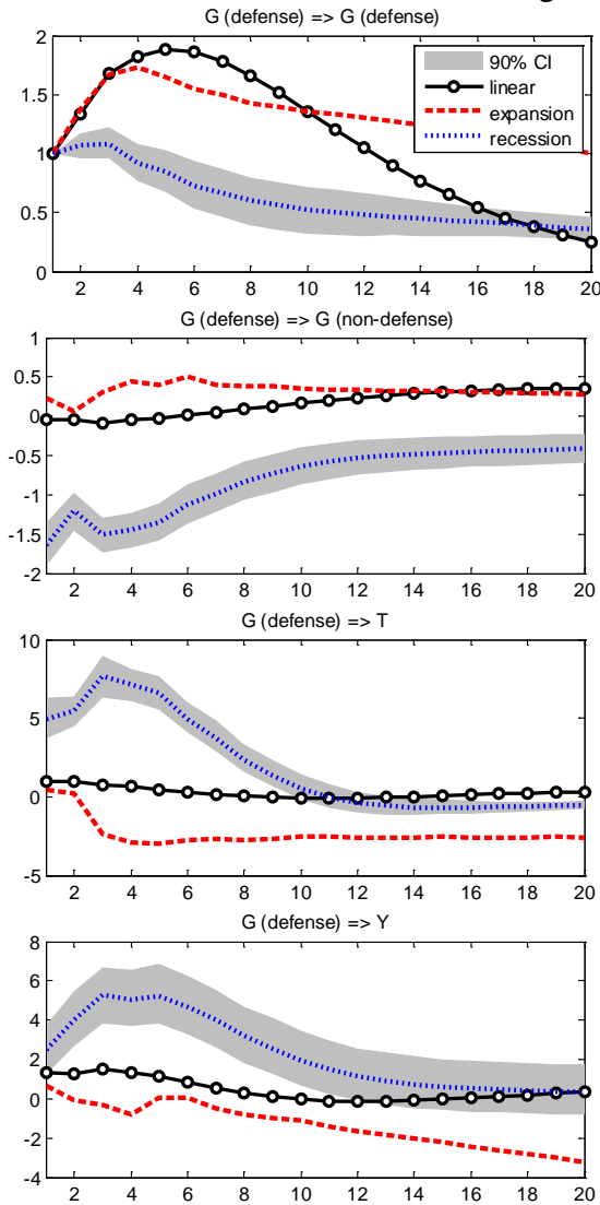
confidence bands for the recession regime
