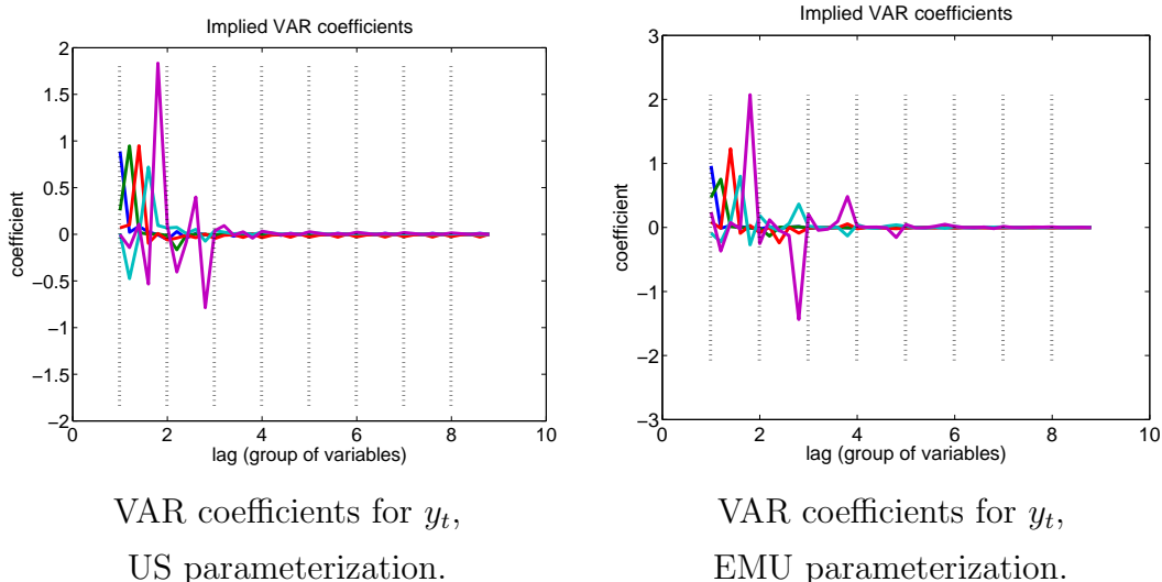
Figure 5: Coefficients in the derived VAR representation for y_t .
