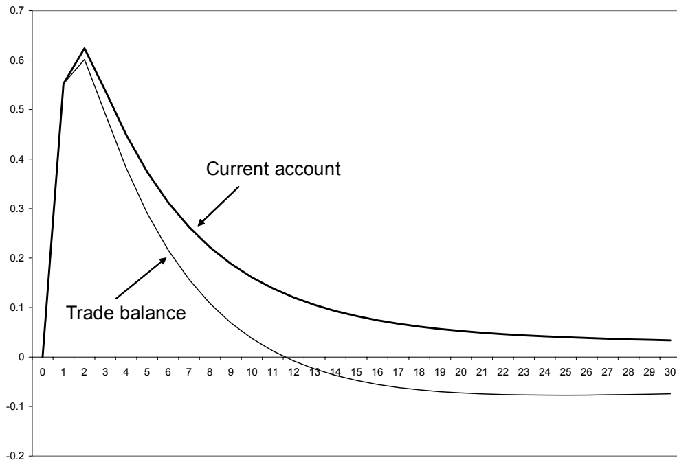
Figure 6. External balances in standard (FDF) model
