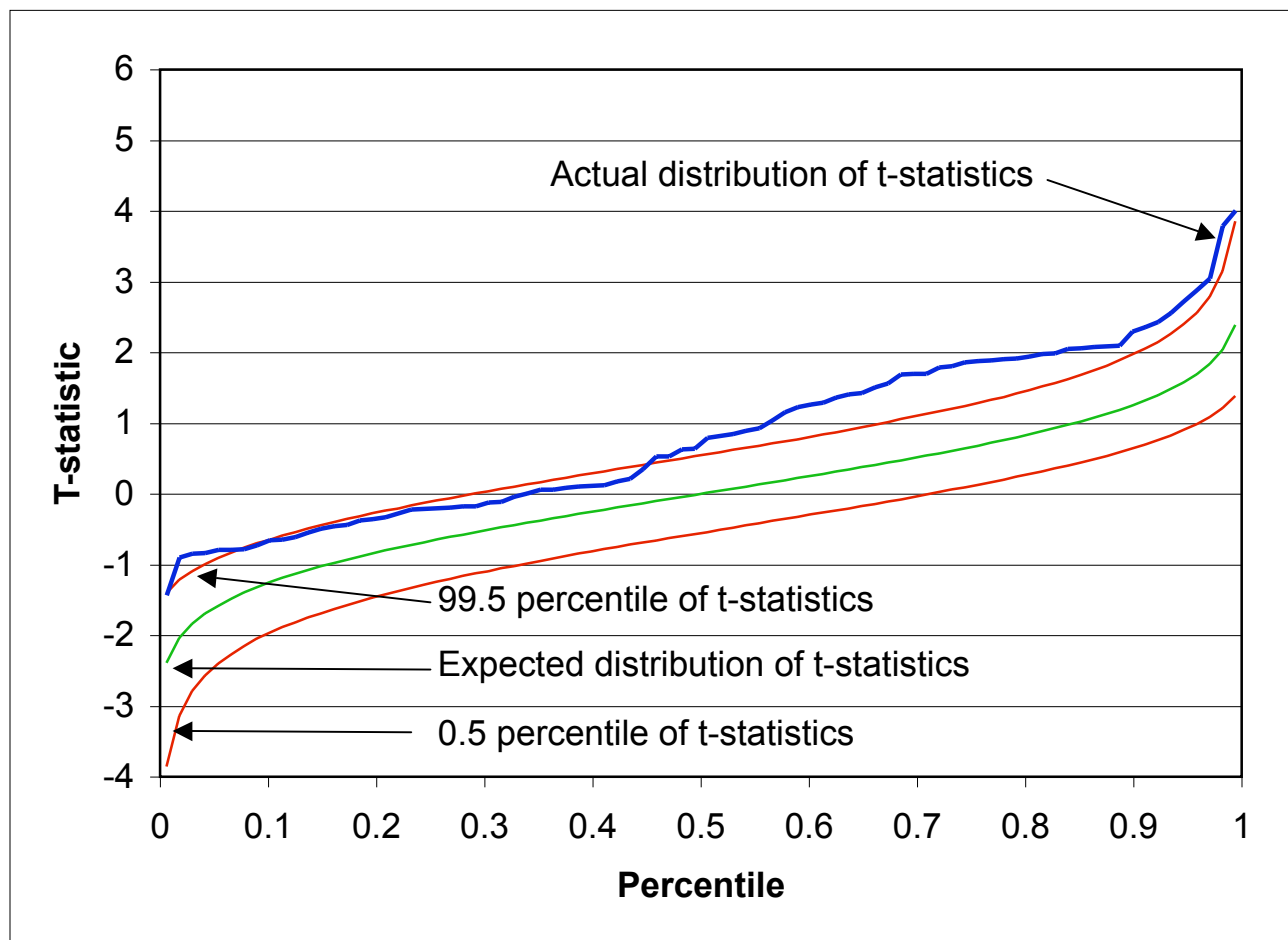
Figure 3: The Actual and Predicted Percentiles of the Distribution of T-statistics for Behavior and Mental and Physical Health Outcomes.
