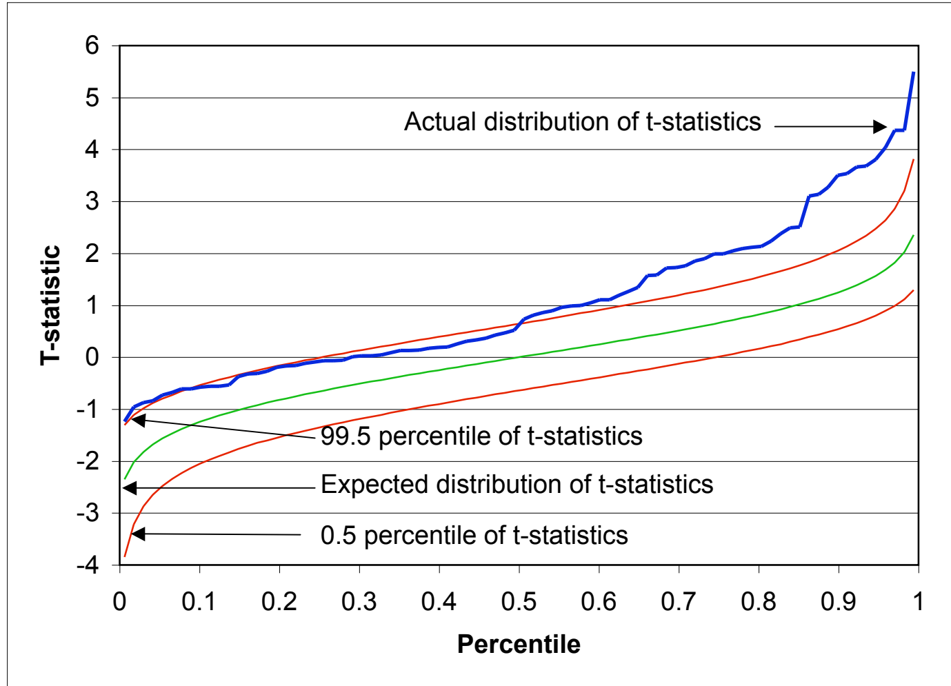
Figure 2: The Actual and Predicted Percentiles of the Distribution of T-statistics for Buffering of Education and Income Outcomes
