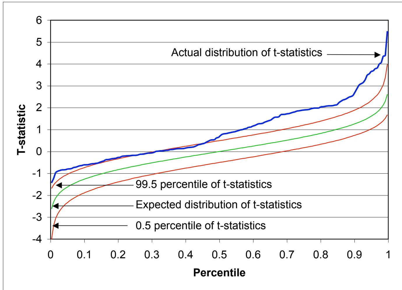
Figure 1: The Actual and Predicted Percentiles of the Distribution of T-statistics
