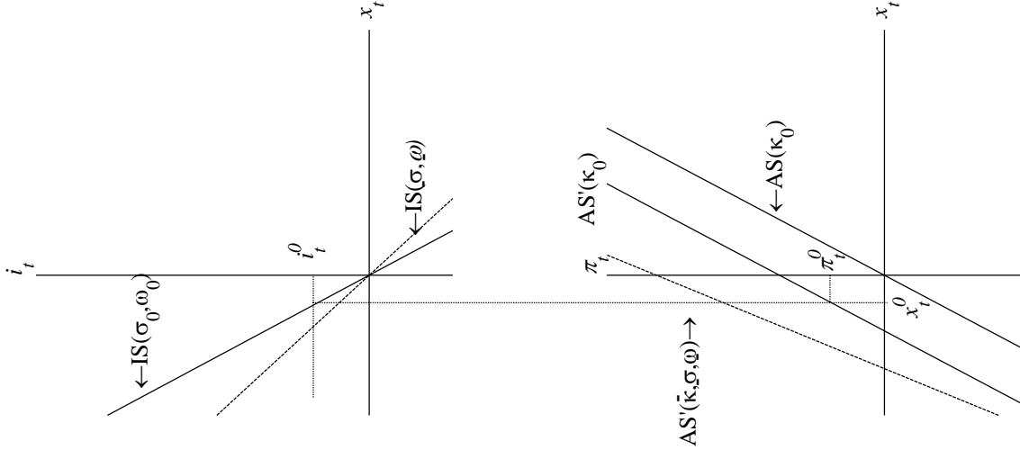
Figure 4c: \mu -shock
