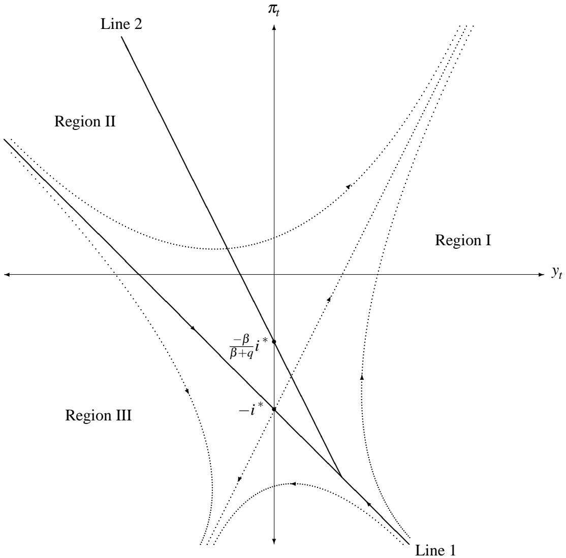
Figure B1: Phase Diagram for the Ball-Svensson Model under Optimal Policy
