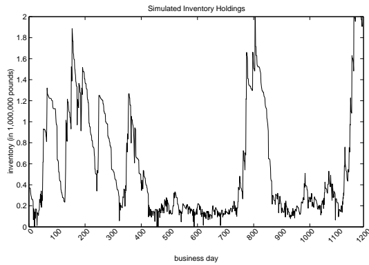
Figure 4: Simulated inventory data from the estimated Figure 5: Censored (solid line) and uncensored (dotted line) purchase prices, p_t from a simulation for product 4.
