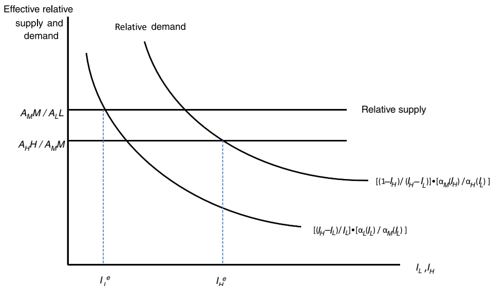
Figure 23 Equilibrium allocation of skills to tasks.
