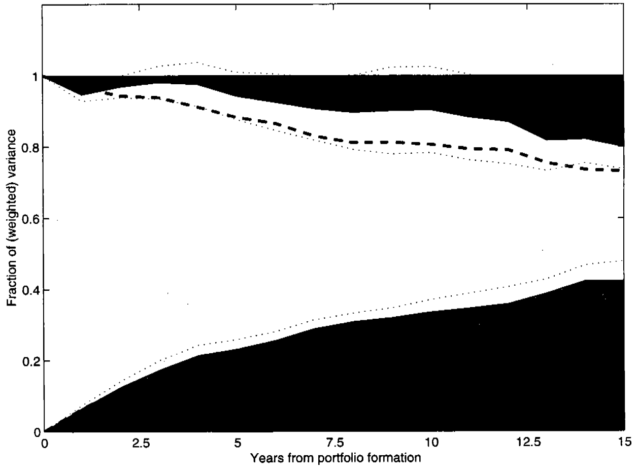
Figure 1: Variance shares for the stock-return CAPM
