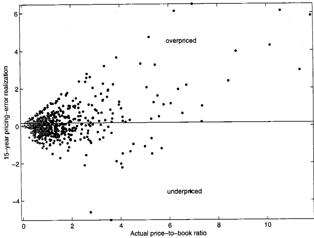
Figure A.2: Realizations of the stock-return CAPM pricing-error component
