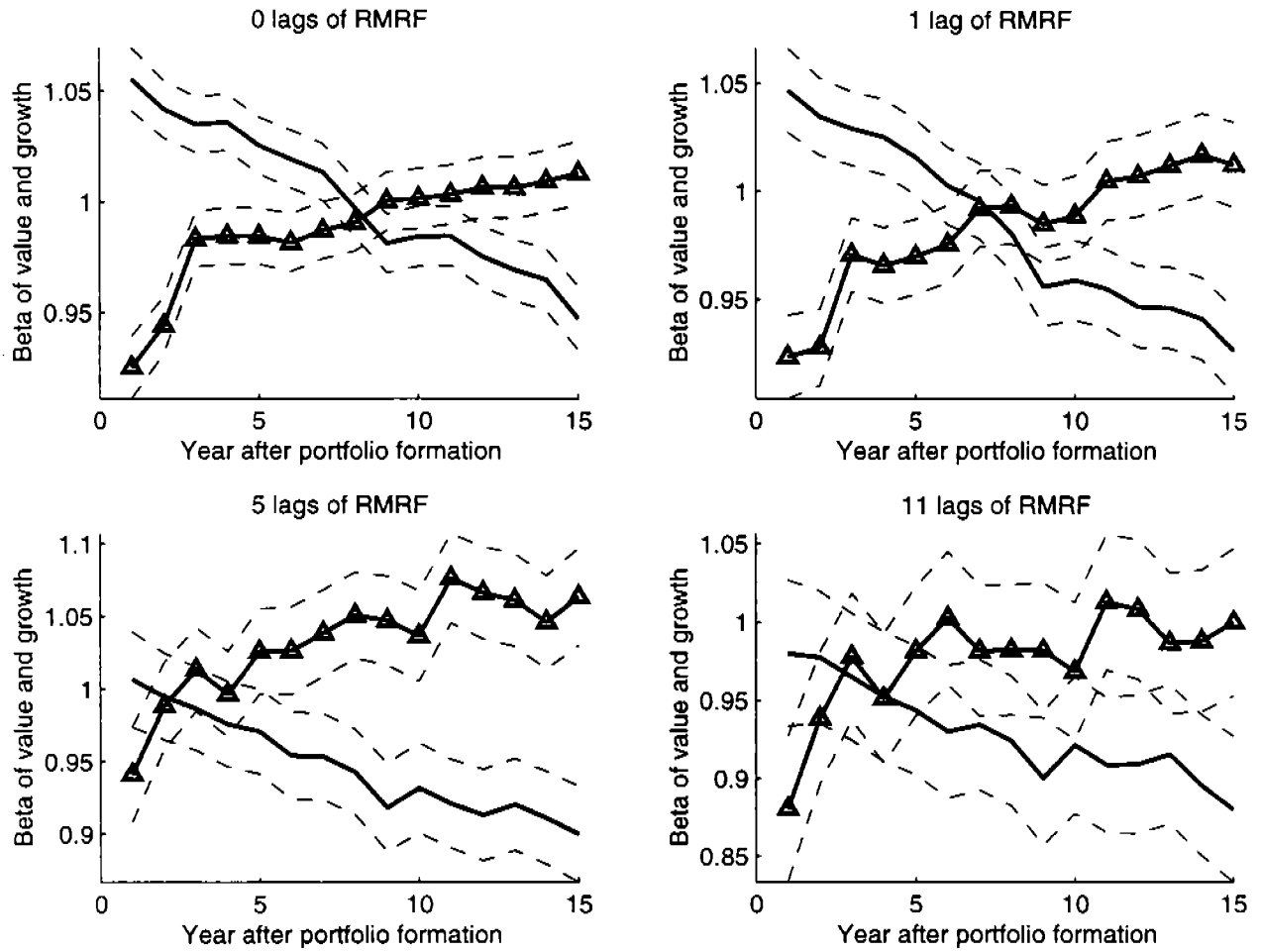
Figure 3: Evolution of the CAPM beta after portfolio formation
