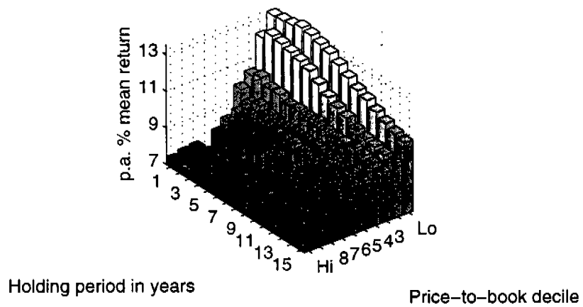
Figure 4: Mean excess returns and alphas for different holding periods
