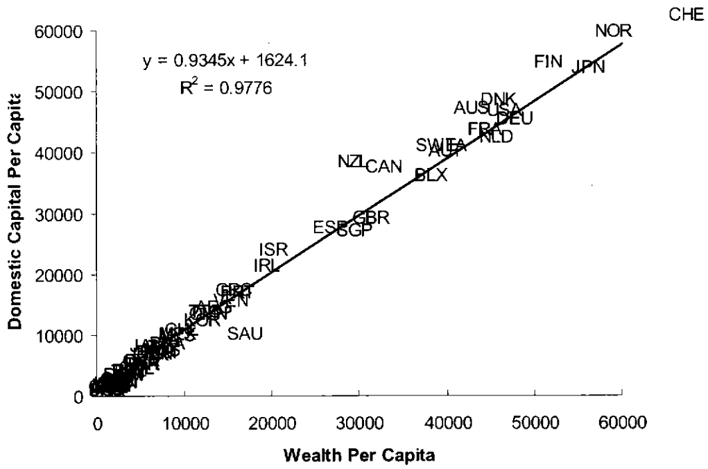
Figure 2: Domestic Capital Stocks and Wealth Are Highly Correlated
