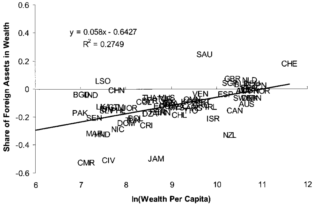
Figure 3: The Share of Net Foreign Assets In Country Portfolios Increases with Wealth
