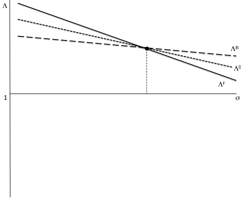
Figure 8: Single crossing between \Lambda^F , \Lambda^B and \Lambda^D
