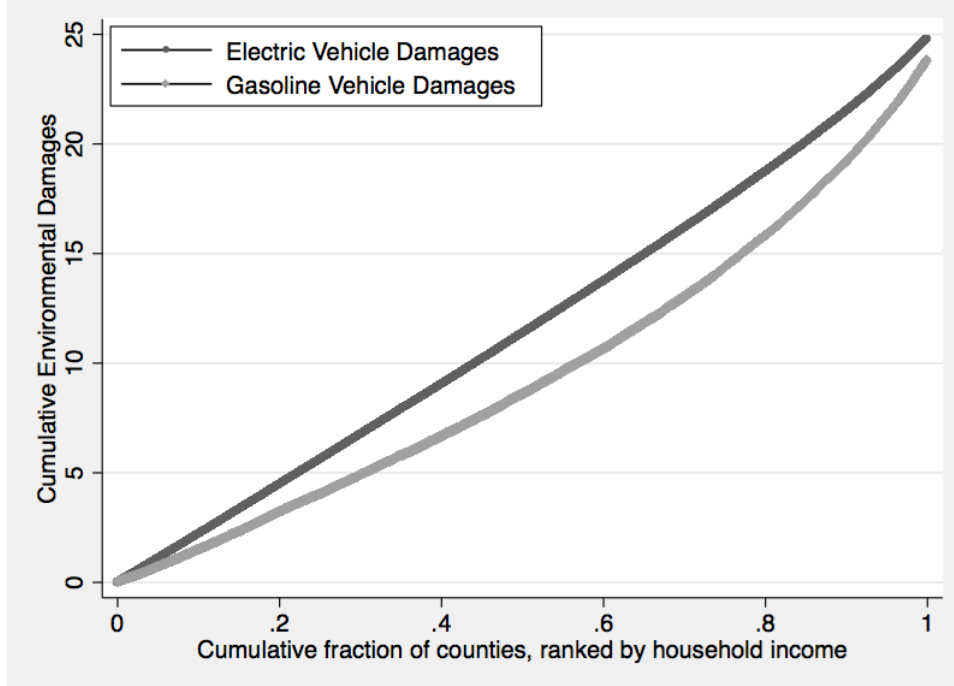
Figure 8: Cumulative Distributions: Air Pollution Damages from Driving
