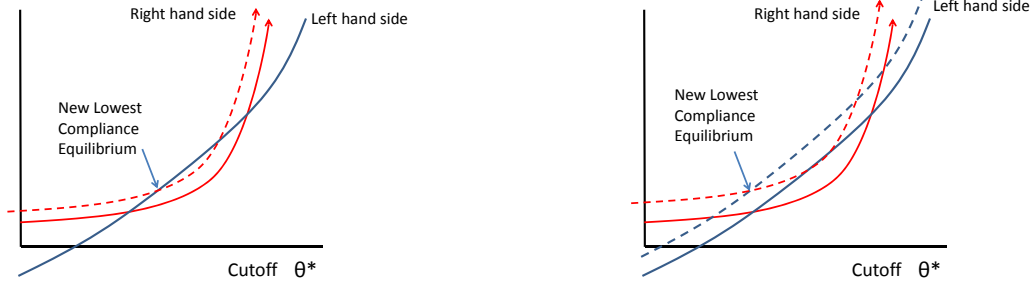
(a) Comparative Statics of the Equilibrium Thresholds due to an increase in fine, public enforcement, or externality.
