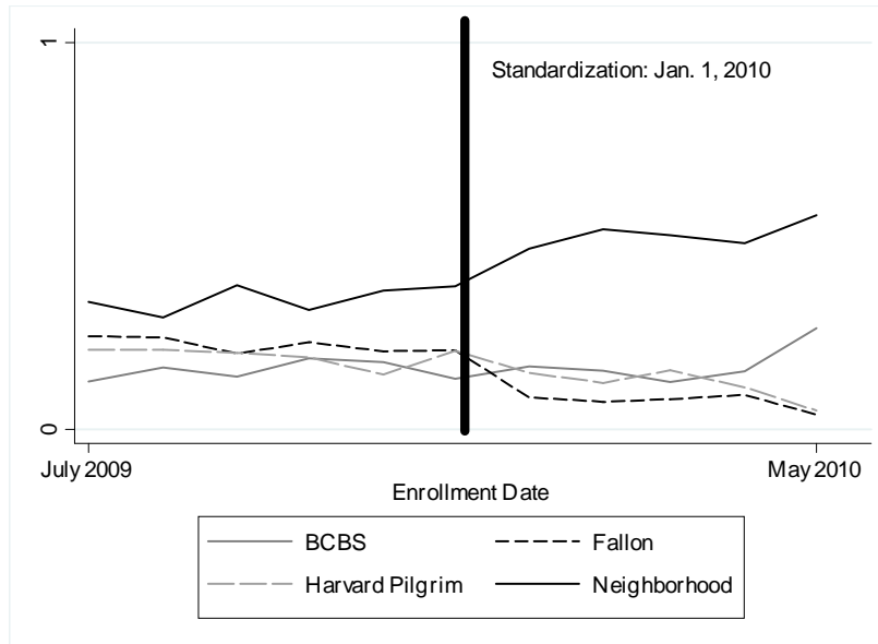
Figure A.1: No Evidence of Time Trends
