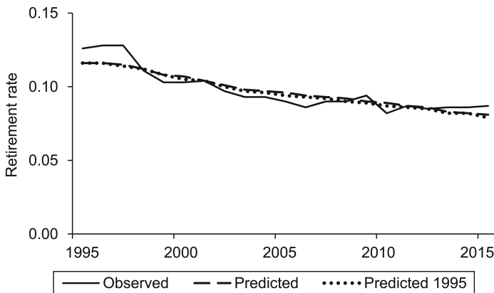
Figure 2.11 Counterfactual simulations
