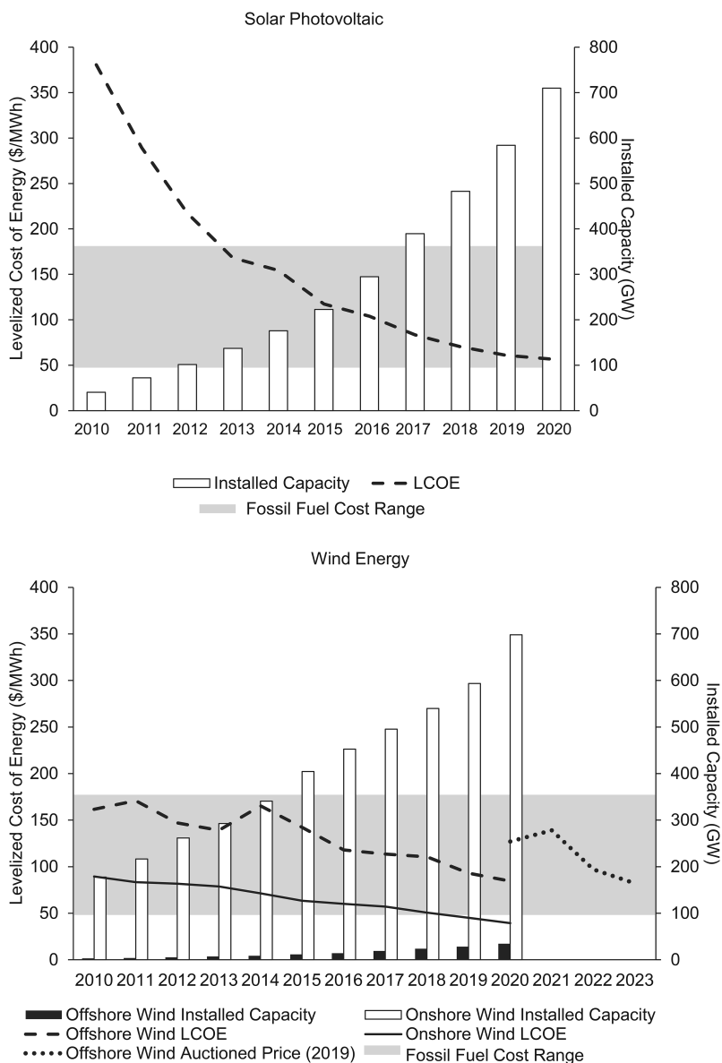
Figure 2.4 The deployment and cost of renewables, 2020 GW
