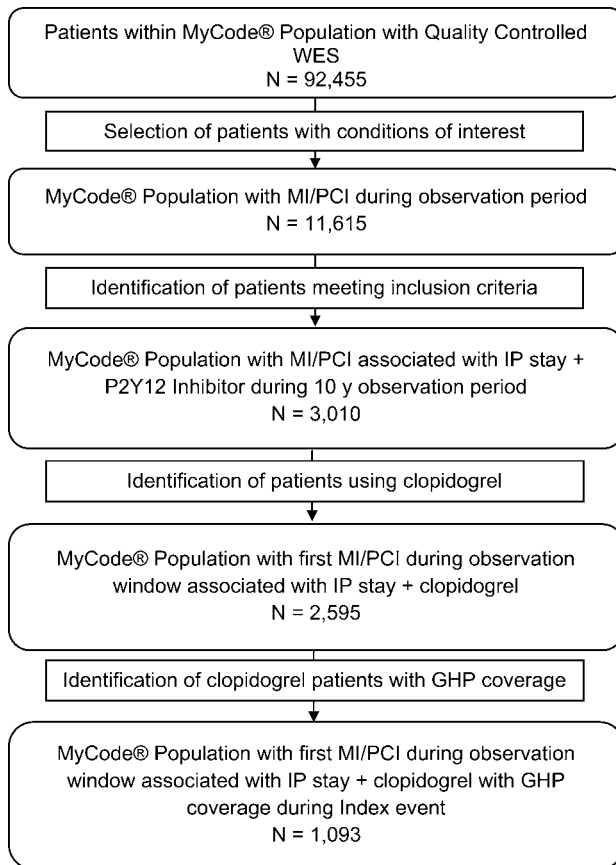
Fig. 10.1 Population selection
