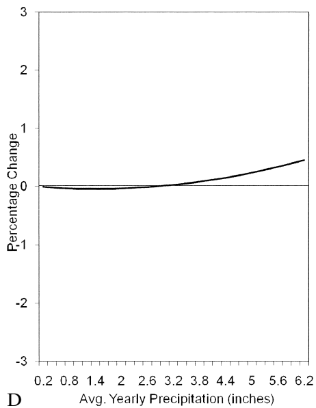
Fig. 4.4 Percent change in cotton price: A , From percent change in local average temperature; B , From percent change in other producers' (OP) average temperature; C , From percent change in local average precipitation; D , From percent change in OP average precipitation
