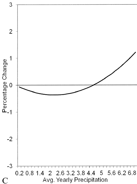
Fig. 4.6 Percent change in hay price: A , From percent change in local average temperature; B , From percent change in other producers' (OP) average temperature; C , From percent change in local average precipitation; D , From percent change in OP average precipitation
