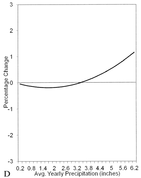
Fig. 4.5 Percent change in corn price: A, From percent change in local average temperature; B, From percent change in other producers' (OP) average temperature; C, From percent change in local average precipitation; D, From percent change in OP average precipitation
