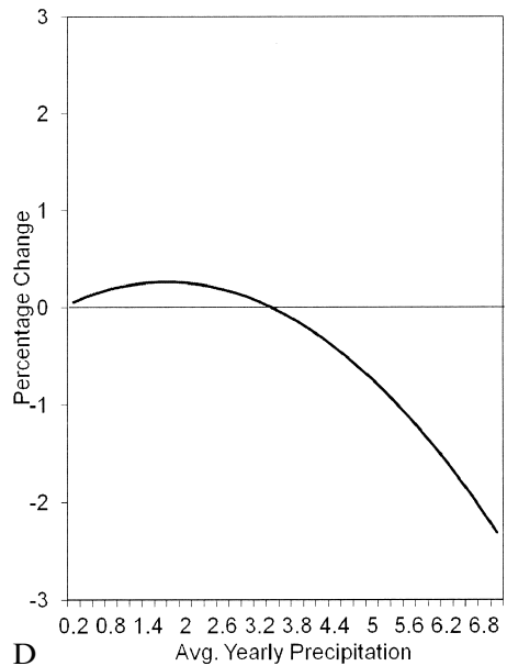
Fig. 4.6 Percent change in hay price: A , From percent change in local average temperature; B , From percent change in other producers' (OP) average temperature; C , From percent change in local average precipitation; D , From percent change in OP average precipitation
