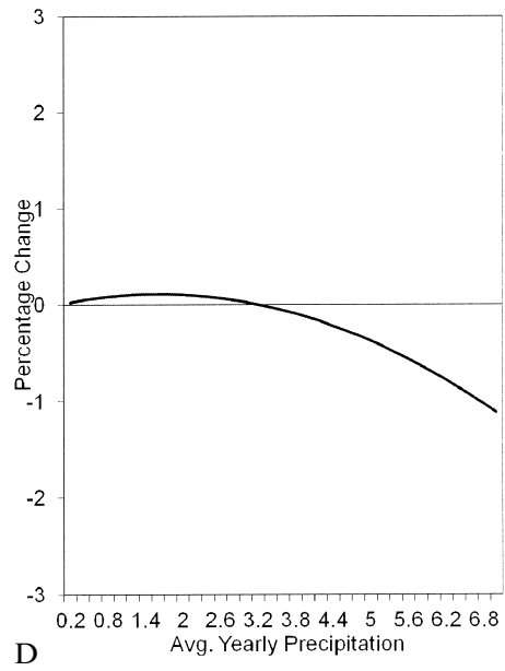
Fig. 4.7 Percent change in wheat price: A , From percent change in local average temperature; B , From percent change in other producers' (OP) average temperature; C , From percent change in local average precipitation; D , From percent change in OP average precipitation
